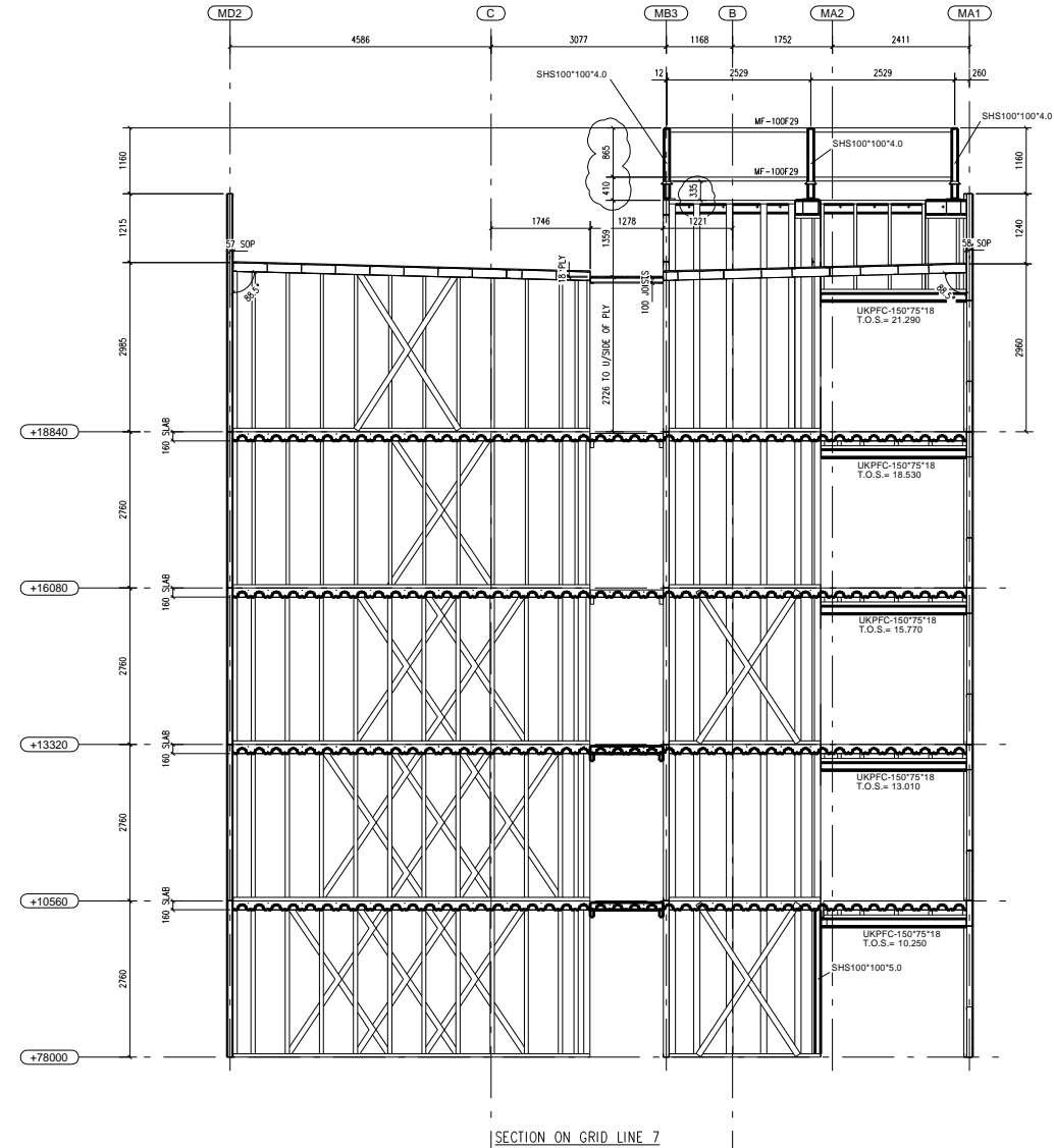
SECTION ON GRID LINE 7
