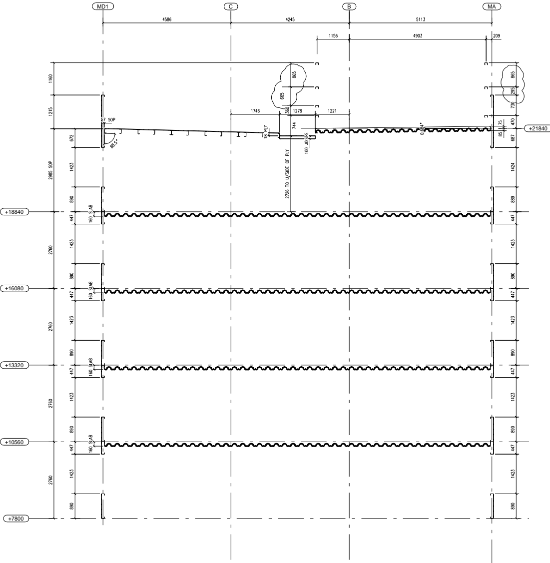
SECTION BETWEEN GL's 4 & 3A
